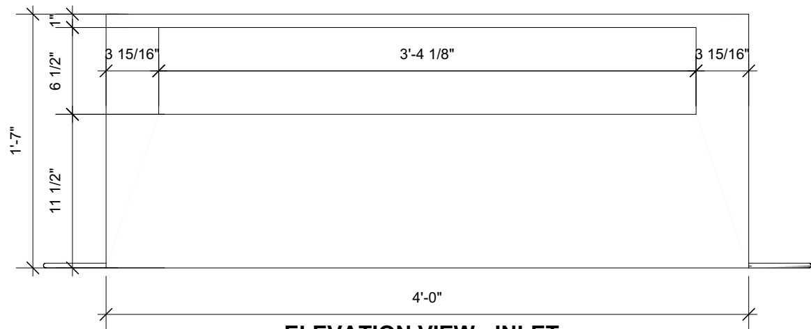
ELEVATION VIEW - INLET
