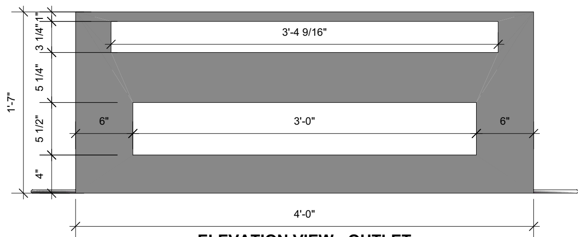
ELEVATION VIEW - OUTLET
