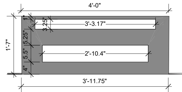
ELEVATION VIEW - OUTLET
